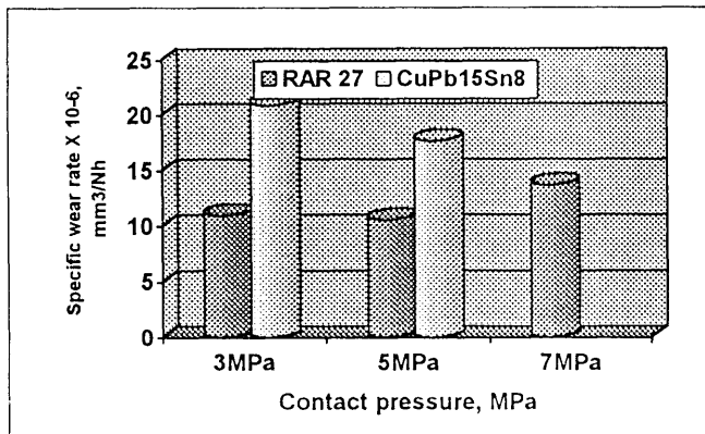
Figure 6. Specific wear rates of tested materials
