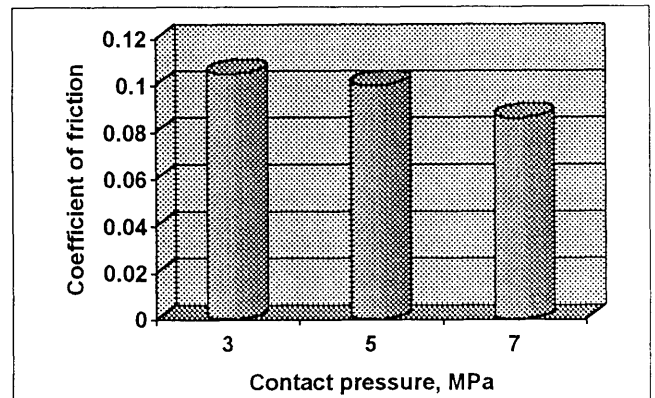
Figure 7. Coefficient of friction vs contact pressure
