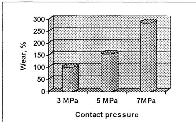
Figure 3. Wear vs contact pressure
