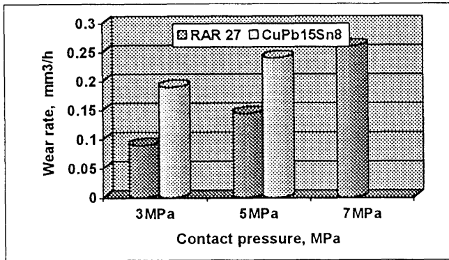
Figure 5. Wear rates of tested materials
