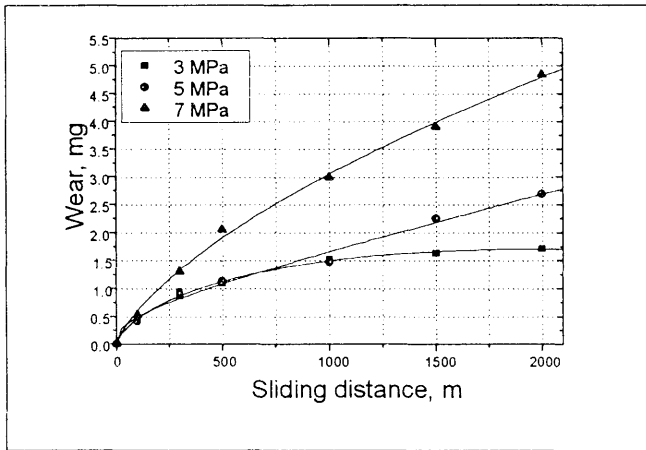
Figure 2. Wear curves
