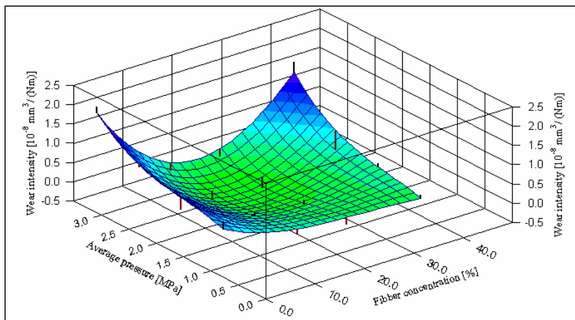
Figure 9. Wear intensity of PTFE + glass fiber composites, after 10500 m of sliding in water at 2.5m/s. [8]
